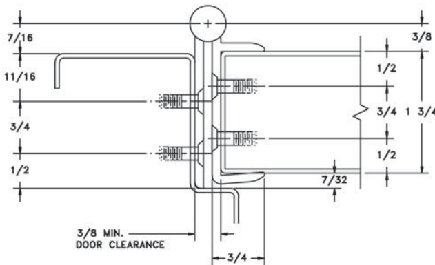
DOOR CLOSED
